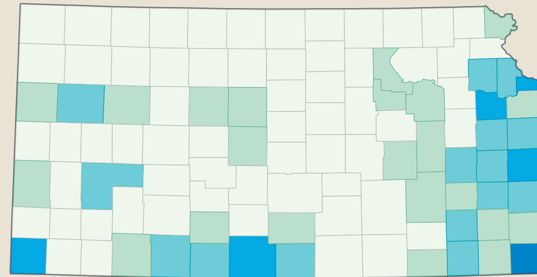
Manual
