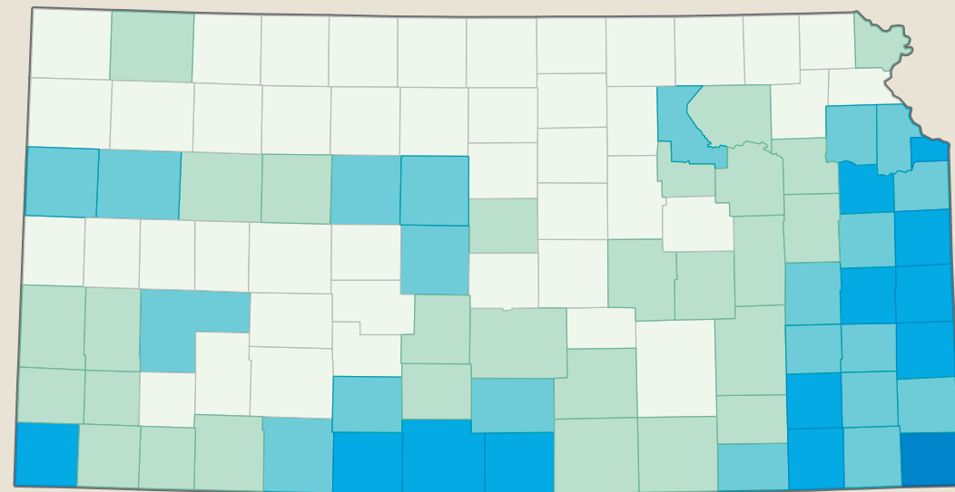
Natural Breaks
