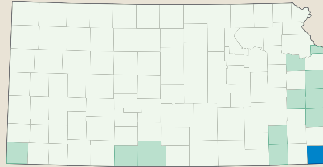
Equal Interval
